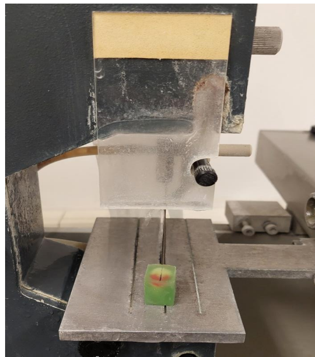
Figure 14. Sample cutting.
