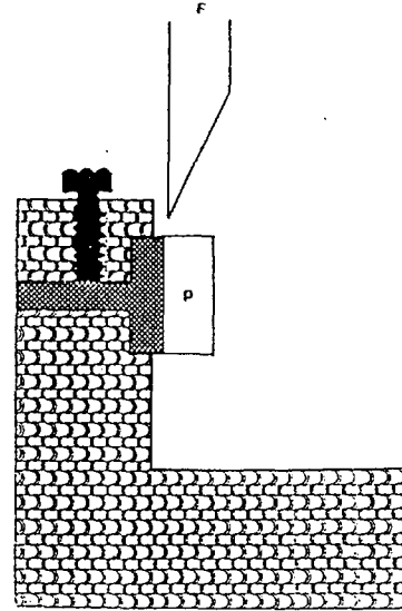
Fig. 1. The scheme of the breaking device placed on the specimen mounted in the holder of the testing machine.
