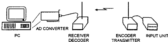
Fig. 1. The entire telemetry system.
