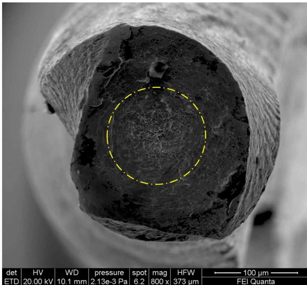
Figure 6. SEM image of the fractured surface of an F-One #20 after torsional testing. The typical features of excessive torsional load, showing concentric circular abrasion marks. Courtesy of Zanza et al. (39).
