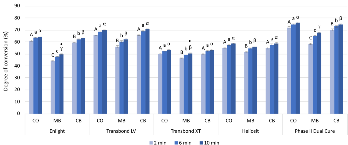
Figure 5. Degree of conversion (mean values and standard deviations) measured 2, 6, and 10 min after light curing for each system. For the comparisons among bracket types, the same uppercase, lowercase, and Greek letters indicate statistically similar values after 2, 6, and 10 min, respectively. Statistically similar values among the materials (within each combination of bracket type and time point) are marked by dots (·). CO: control group (no bracket); MB: metal bracket group; CB: ceramic bracket group.
